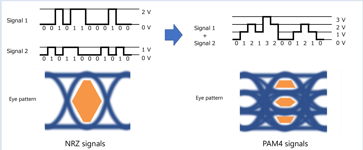
Figure 4. NRZ and PAM4 Signals
